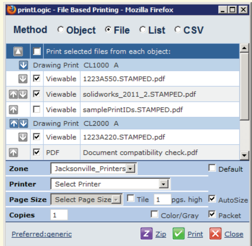
Proprietary Multi-Function Web User Interface
