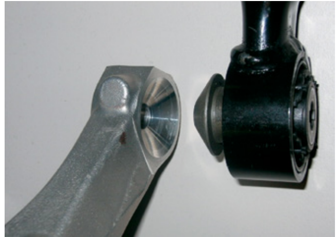
Figure 1. Close-up view, before assembly, of the toe-link (black) and the rear knuckle (silver) using a conical joint.
