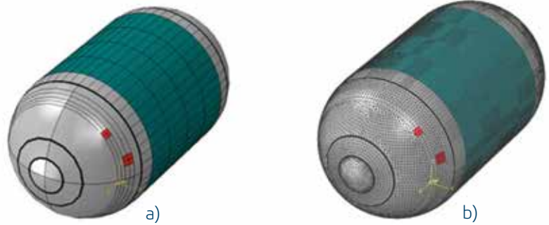
Figure 1. Inflatable plug prototype (left), and Abaqus model of the initial geometry: a) geometry b) meshed.
