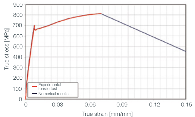
Strong agreement between experiment and Abaqus FEA (numerical) results under tensile tests.
