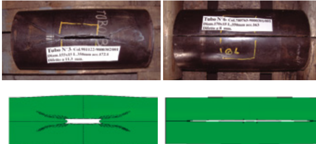
High-toughness (HT) steel burst test and Abaqus/Explicit model (left upper and lower) and low-toughness steel and Abaqus/Explicit model (right upper and lower).
