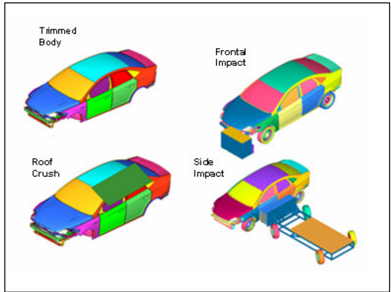
Figure 3: Types of FE Models
