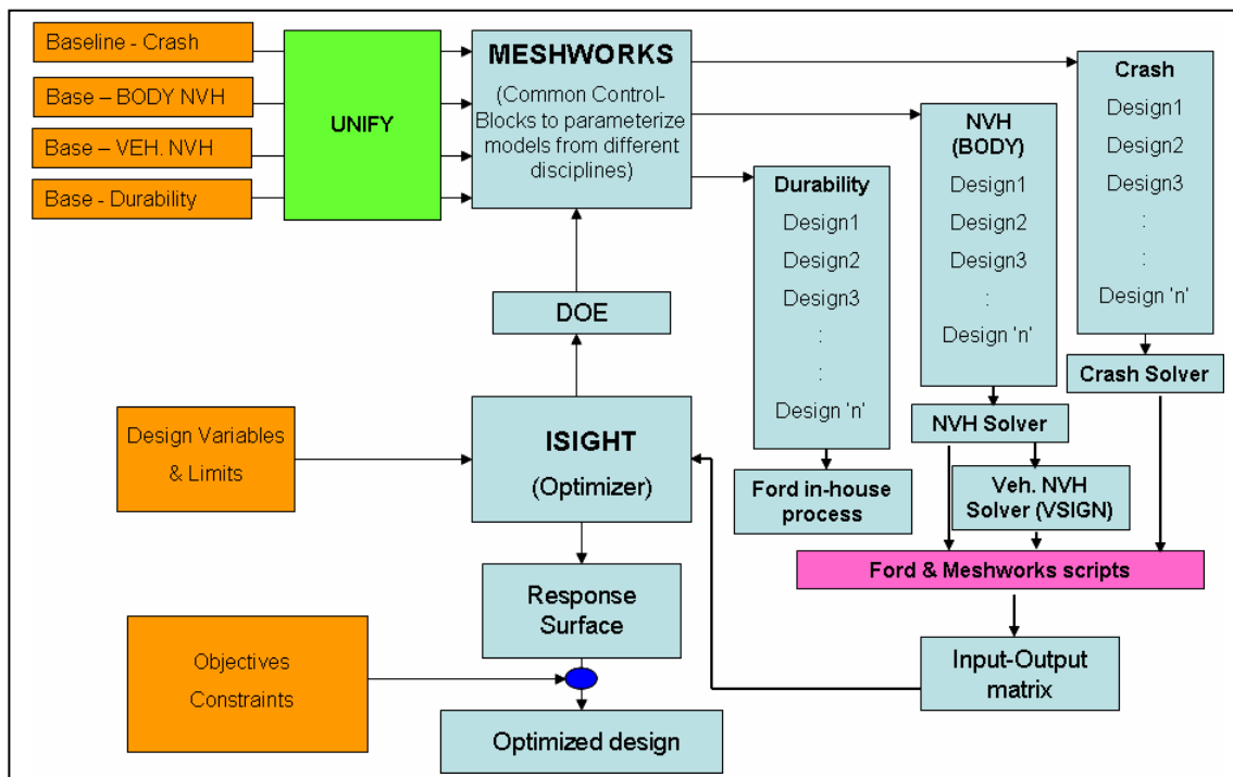
Figure 1. Process flow for Automated MDO Process
