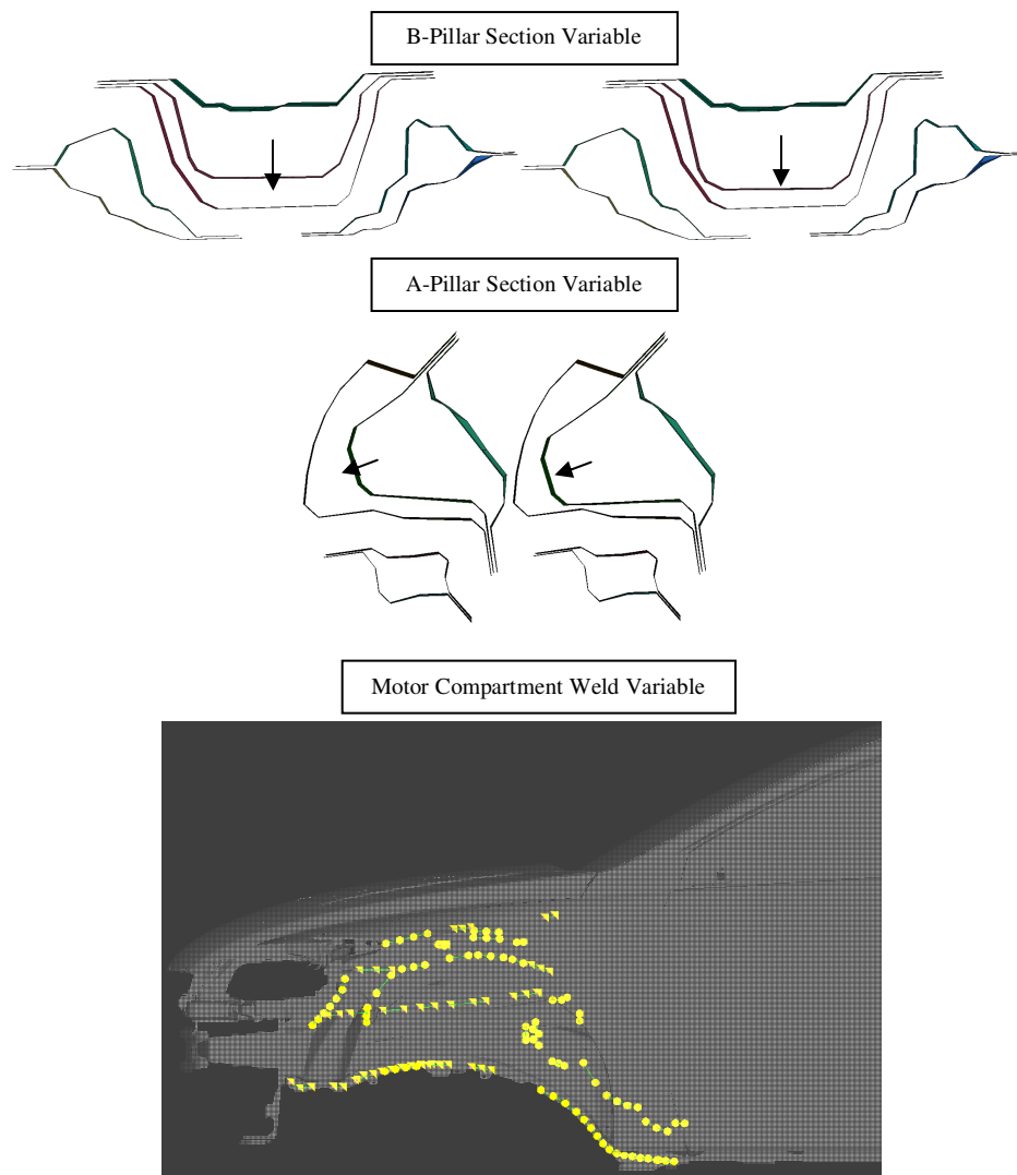
Figure 2: Design Variables
