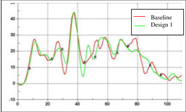
Figure 6: Acceleration Response
