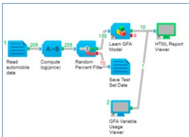
Figure 1. An example machine learning protocol
