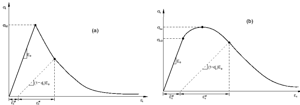
Figure 5. Uniaxial loading in the CDP model in (a) tension and (b) compression
