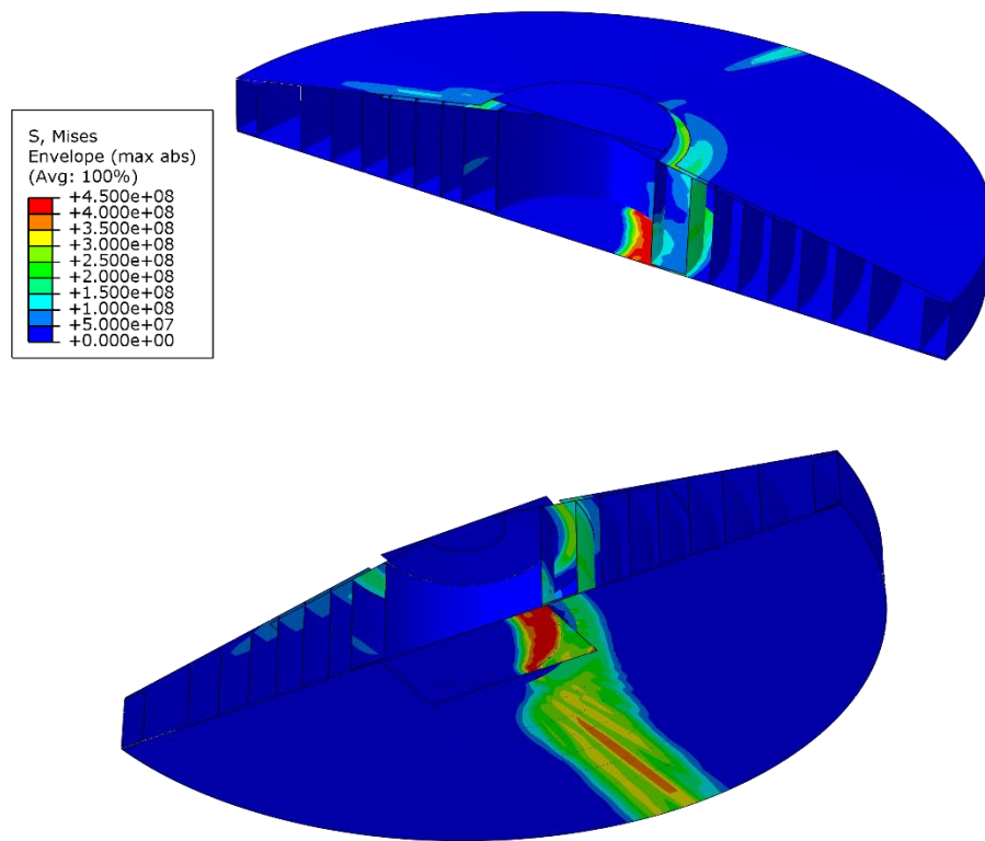
Figure 12. Stresses in the reinforcement (Pa).
