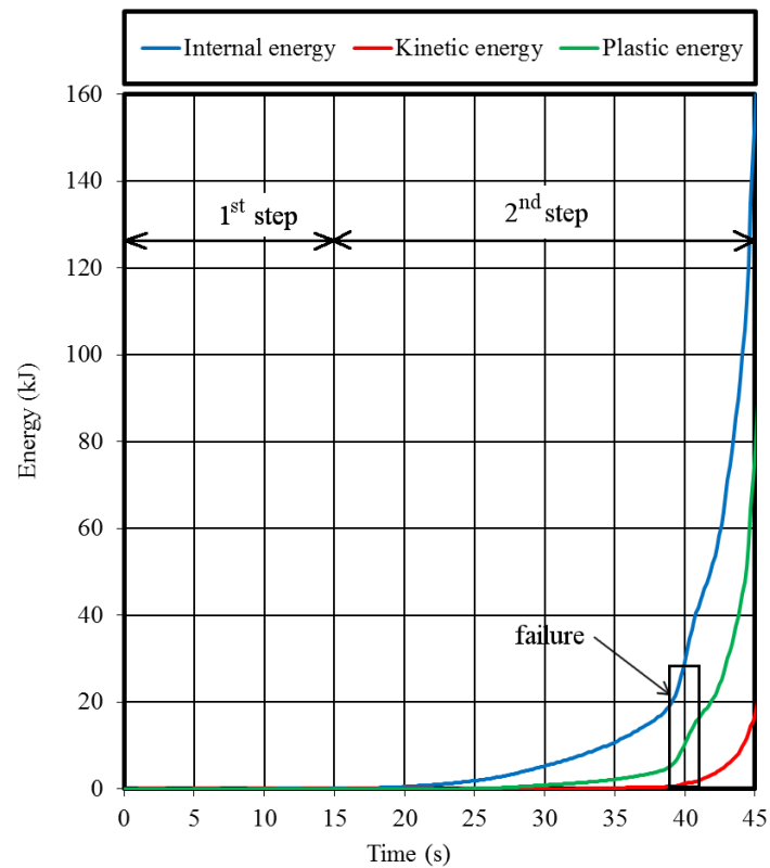
Figure 7. Evolution of energies during the loading process.
