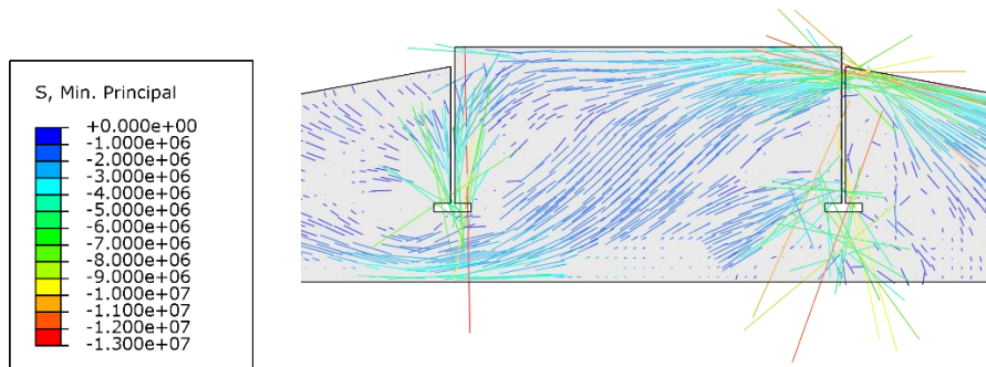
Figure 10. Direction of compressions (Pa).
