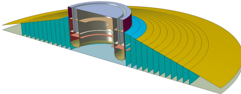
Figure 2. Surfaces with rebars embedded in the concrete.
