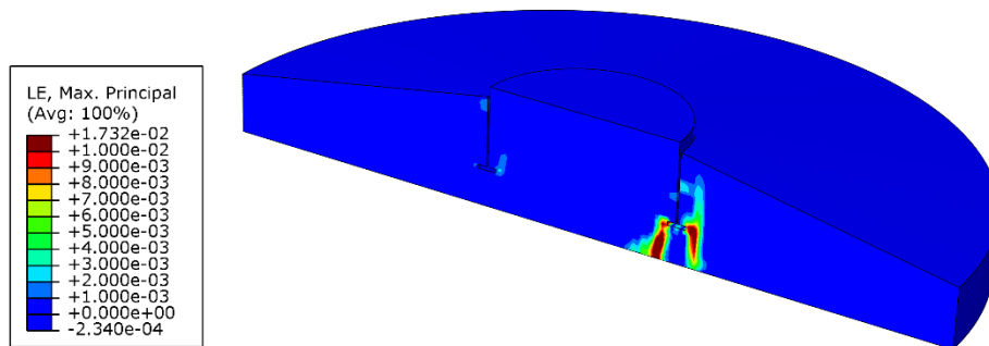
Figure 11. Maximum strains (-).
