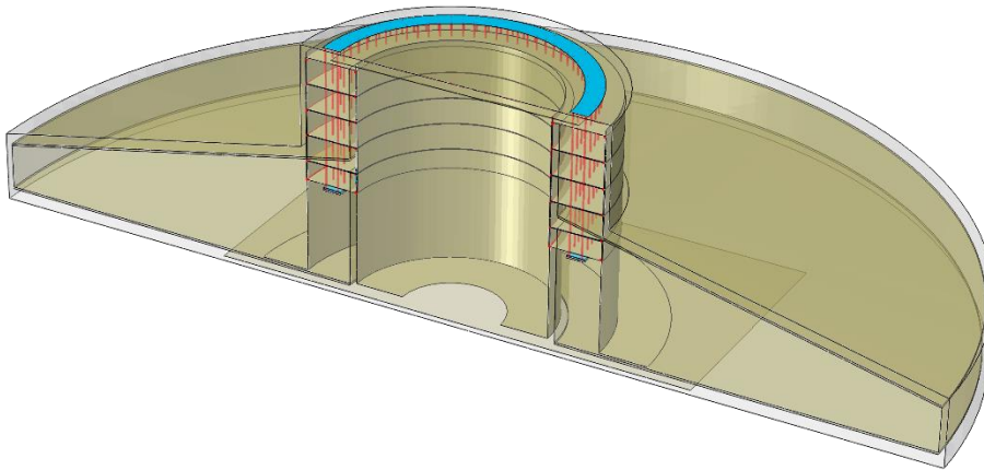
Figure 4. Geometry of a foundation with post-tensioned bolts.
