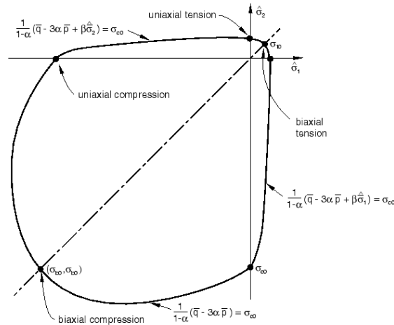
Figure 6. Yield surface in plane stress.
