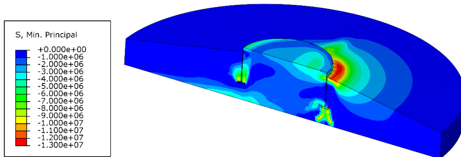
Figure 9. Compression in concrete (Pa).
