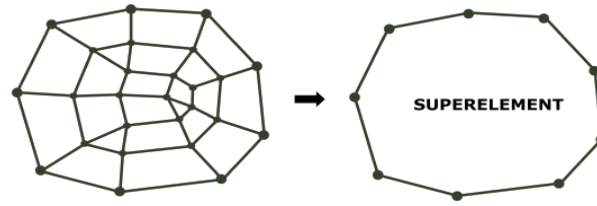
Figure 1. Superelement
