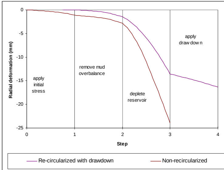
Figure 5 Deformation of the wellbore with and without re-circulatization
