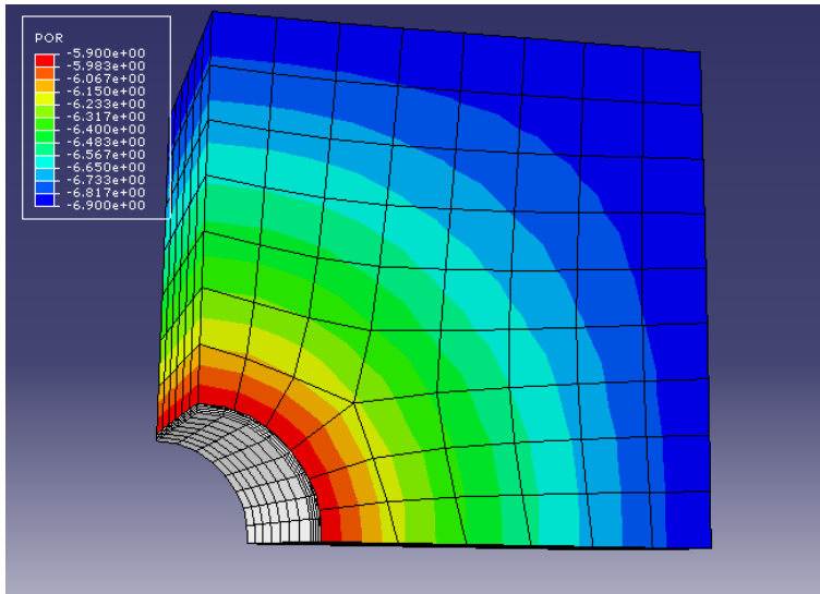
Figure 6 Quarter symmetry model used in the simulations
