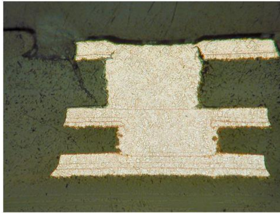
Figure 7: Copper filled microvia with corner crack. Source: Paul Reid 7
