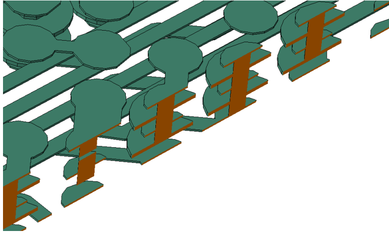
Figure 3: Detailed geometry of vias.
