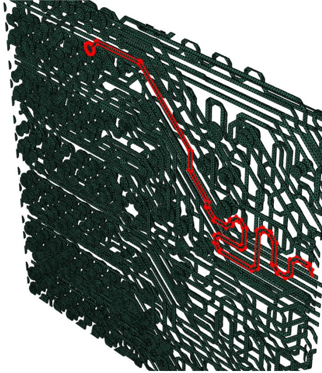
Figure 2: Detailed geometry and mesh of trace.
