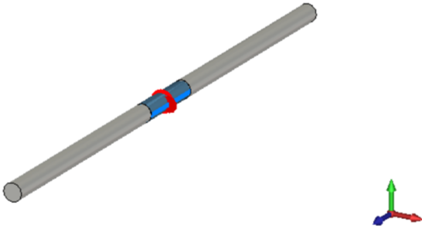
Figure 11: Final model of a half wavelength dipole antenna at 1 GHz
