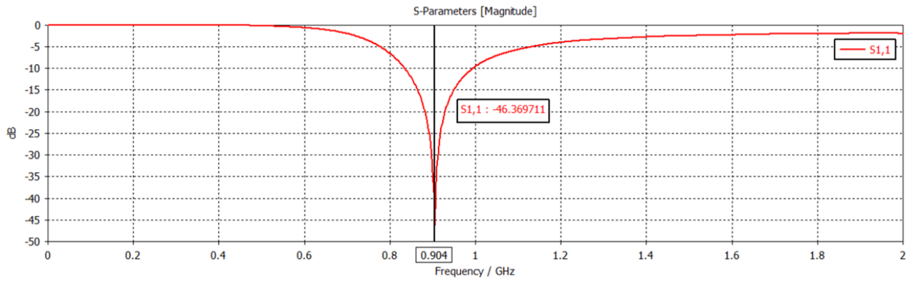
Figure 12: S-parameter result for L = 150 mm of the final model. An additional tweaking should be done in order to move the minimum to 1 GHz.
