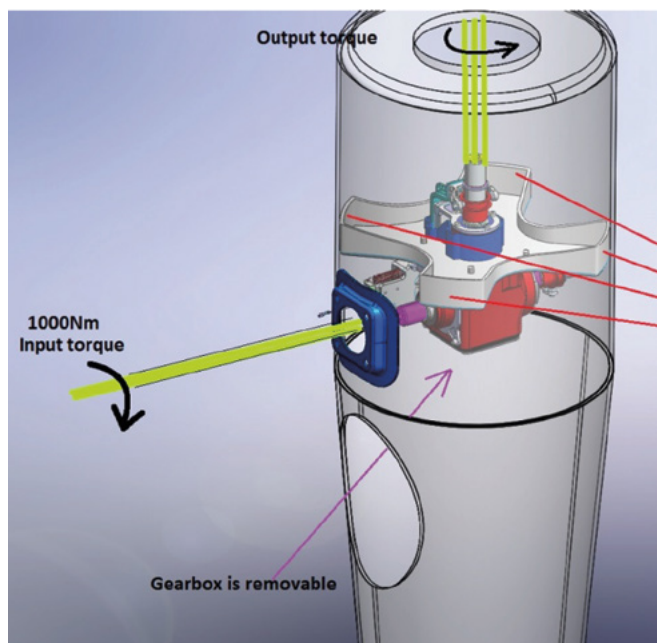
Winch gear (red) and support (grey and white) inside shaft. Winch (not shown) is at top.
