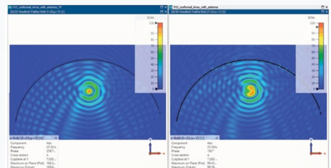
Figure 6: Electric field visualization for solid model (left) and Thin Panel (right) at f=25 GHz.
