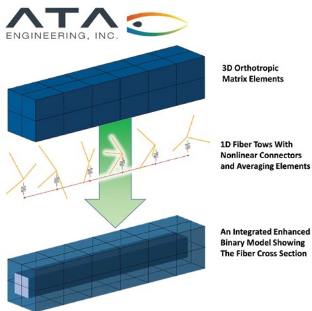
Figure 1. The EBM formulation for composite material architectures.
