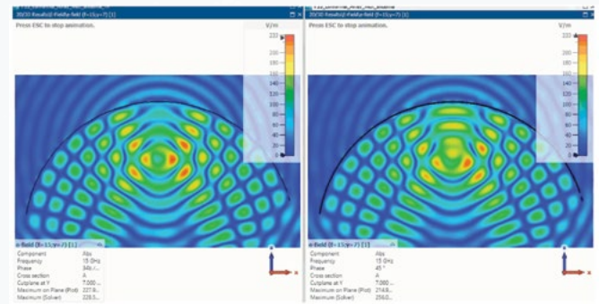
Figure 5: Electric field visualization for solid model (left) and Thin Panel (right) at f=15 GHz.
