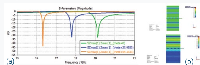
Figure 2. a) Reflection coefficient of the infinite array based on different angle of incidence, b) Electric field animation at transparent and opaque frequencies of the unit cell.
