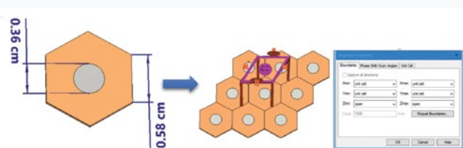
Figure 1. Unit cell structure; Floquet mode analysis of infinite array with the help of Unit Cell Boundary condition provided inside Frequency domain Solver.
