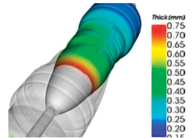
Ever wondered what the inside of a blow mold or injection mold look like during filling? With Abaqus, you can visualize exactly what's going on.
