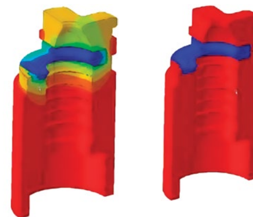
Abaqus can also be used to simulate the manufacturing process. Here, the effects of inadequate mold insulation are easily visualized—on the left is a tool with no insulation, while the right shows one that's been fully insulated.
