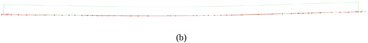
Figure 9.a) Thin wall thermal contour plots at various stages during printing; b) Final deformed configuration (red - experimental bottom surface vs. green – simulation result for the build plate).
