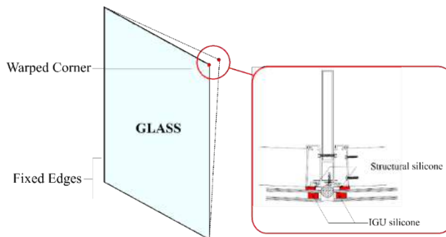
Figure 4: The connection detail
