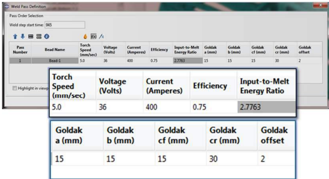
Figure 5 Step Weld Dialog.
