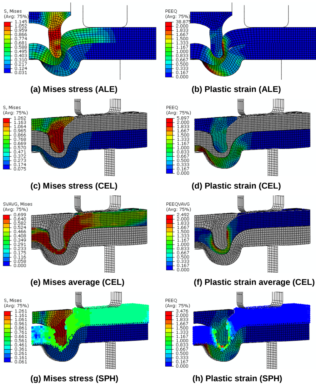
Figure 10. Results of SPFC590.
