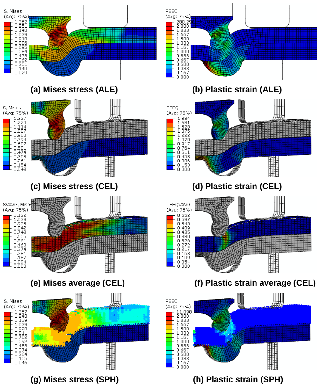
Figure 11. Results of SPFC980.
