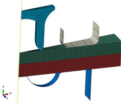
Figure 6. Dummy SPH model
