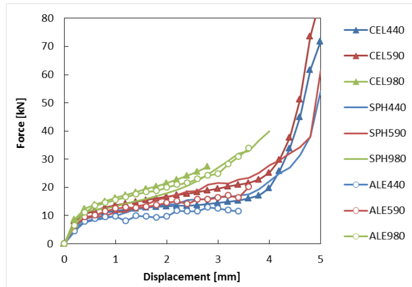
Figure 8. Punch force versus displacement
