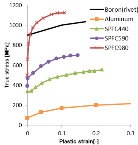
Figure 3. Flow stress curves
