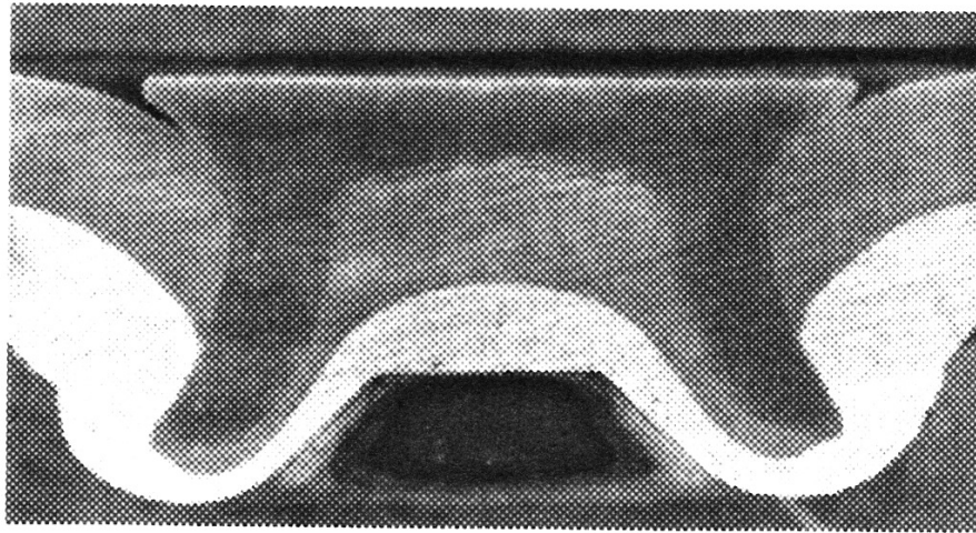
Figure 1. Cross section for experimental SPR forming of 1.4mm SPFC440 (upper sheet) and 1.5mm Aluminum (lower sheet) (Mori, 2014).
