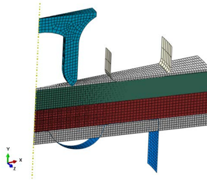
Figure 5. CEL model
