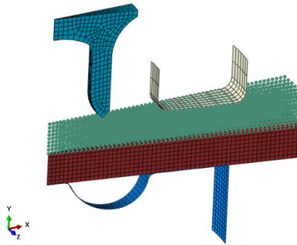
Figure 7. Essential SPH model
