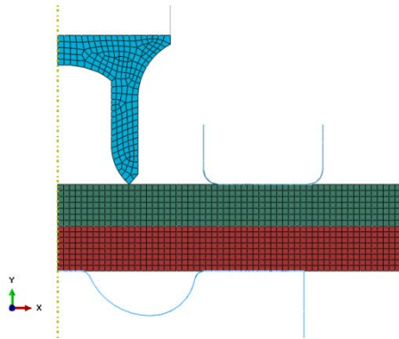
Figure 4. ALE model
