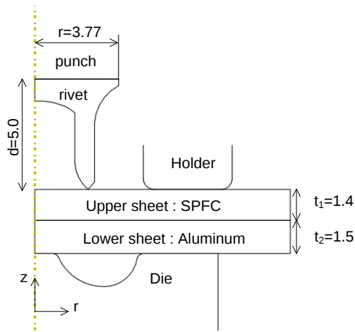
Figure 2. Axisymmetric section
