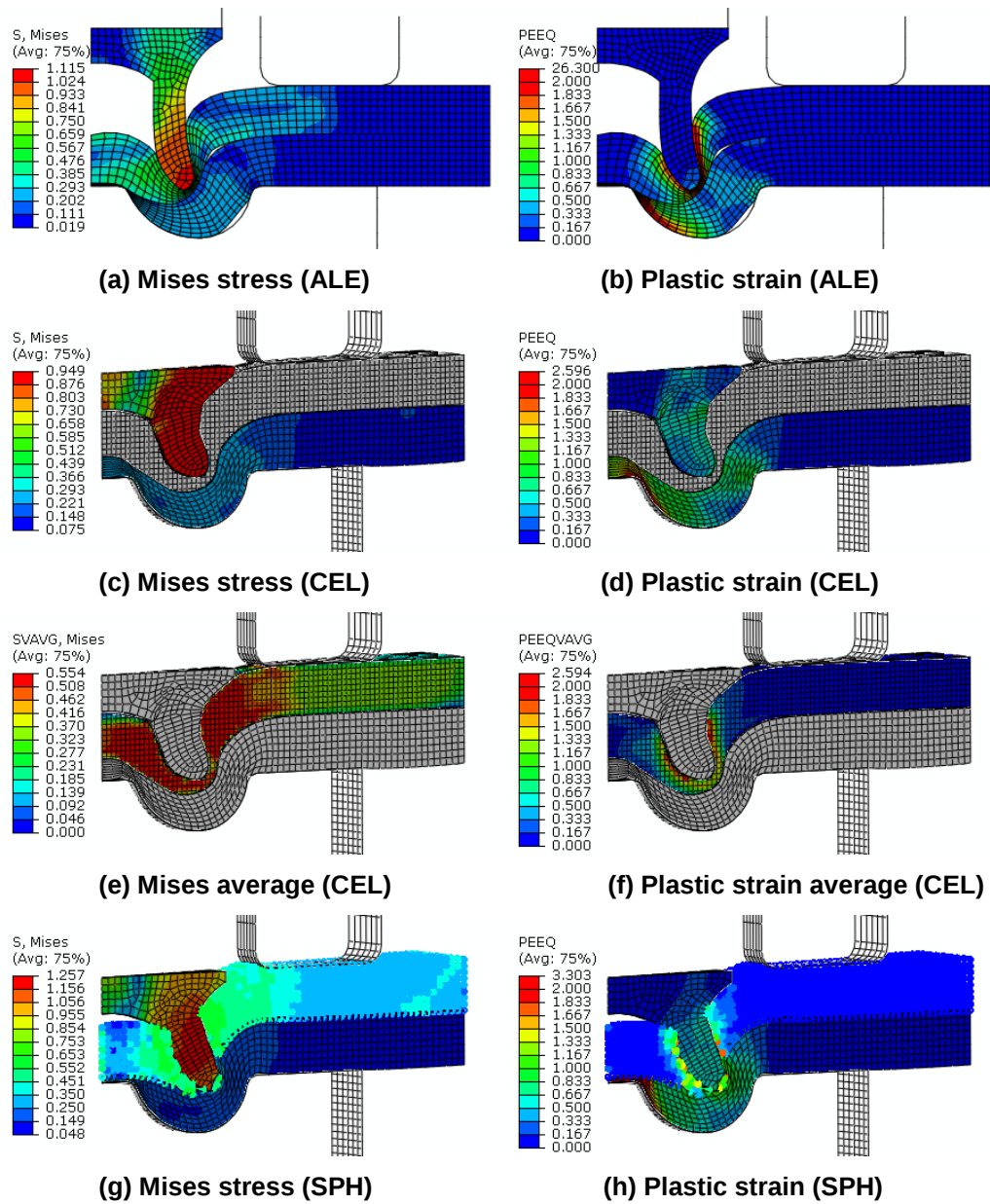
Figure 9. Results of SPFC440.
