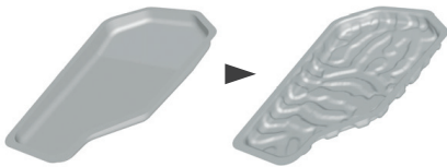
Figure 4: Bead optimization—Efficient bead patterns for increased stiffness and reduced noise
