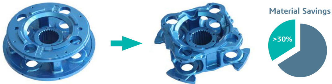
Figure 8: Optimization result of the Voith planet carrier using SIMULIA Tosca Structure
