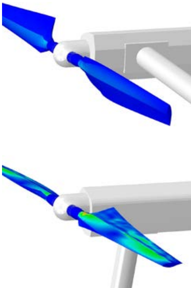
Figure 2, 3. Stresses on outer composite layer of flexible wind turbine blades at different points in time during the emergency brake maneuver. Images courtesy Stefan Sicklinger
