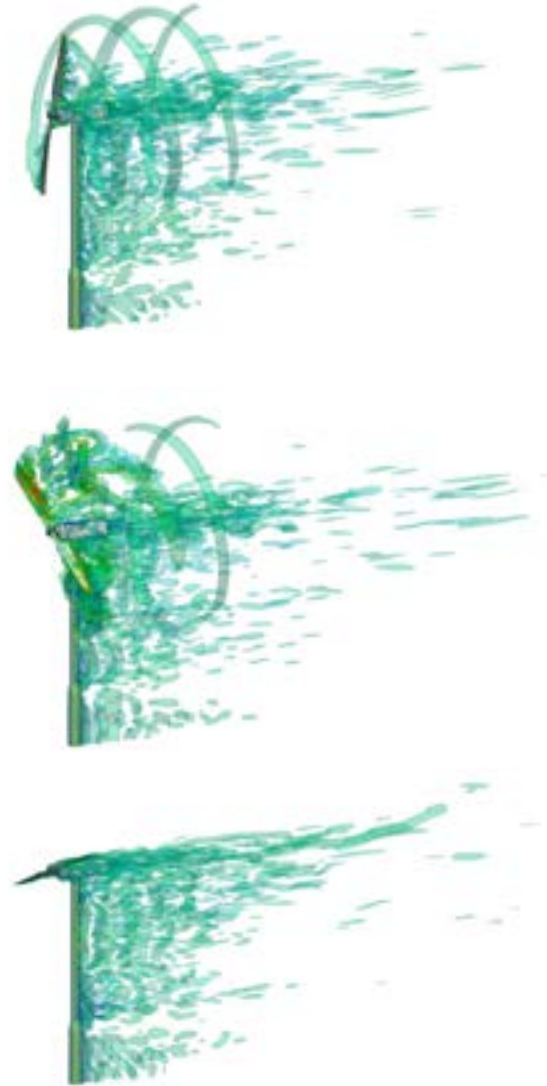
Figure 4-6. Wind turbine simulation showing normal operation (Figure 4), during emergency brake maneuver (Figure 5) and after emergency brake maneuver at standstill (Figure 6). Images courtesy Stefan Sicklinger .
