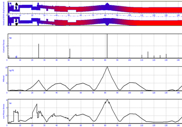
Figure 1. BHA Static Analysis Results.
