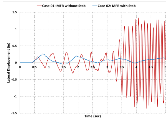
Figure 9: Lateral vibrations at middle of the RSS shaft for vertical orientation.
