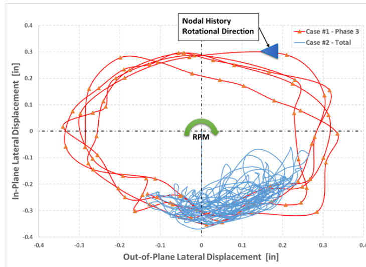
Figure 11: Lateral displacement history at center of RSS pivot stabilizer for Case #1 and full nodal history for Case #2.
