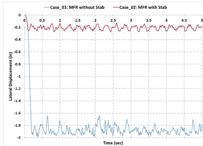
Figure 6. Lateral vibrations for horizontal BHA case at end of MFR unit. The larger lateral displacement of the MFR without stab case is due to MFR sagging as a result of gravity.
