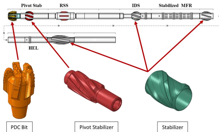
Figure 9. BHA model with location of 3D geometry parts.
