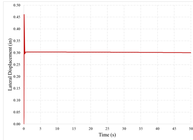
Figure 7. Lateral displacement results for beam elements at center of RSS shaft using time domain method.
