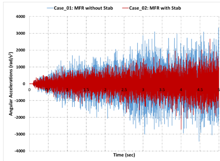
Figure 7. Angular accelerations at center of RSS shaft.
