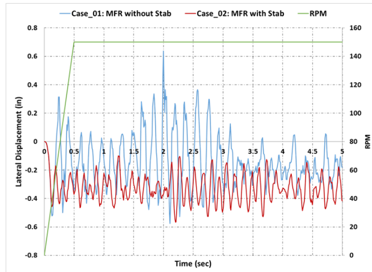
Figure 5. Lateral vibrations (y-axis) for horizontal BHA case at middle of RSS point.
