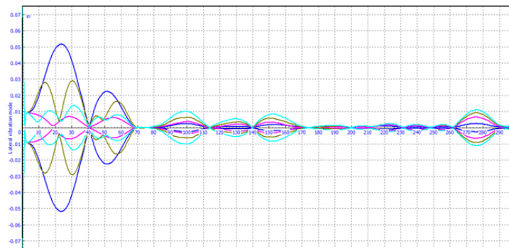
Figure 2. Results of Linear Vibration Analysis.
