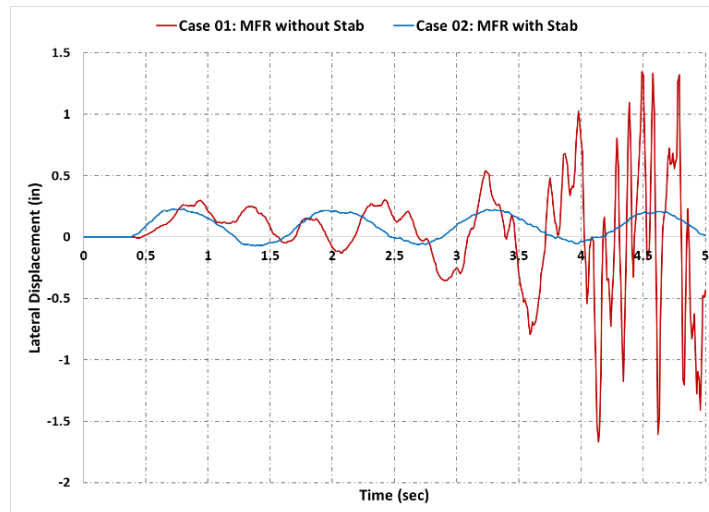
Figure 10: Lateral vibrations at end of MFR unit for vertical orientation.
