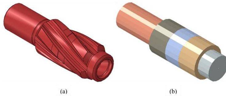
Figure 6. a) Actual pivot stabilizer geometry; (b) Beam element representation.
