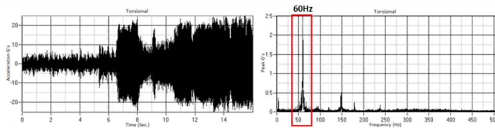
Figure 12: Rapid sample data showing HFTO.
