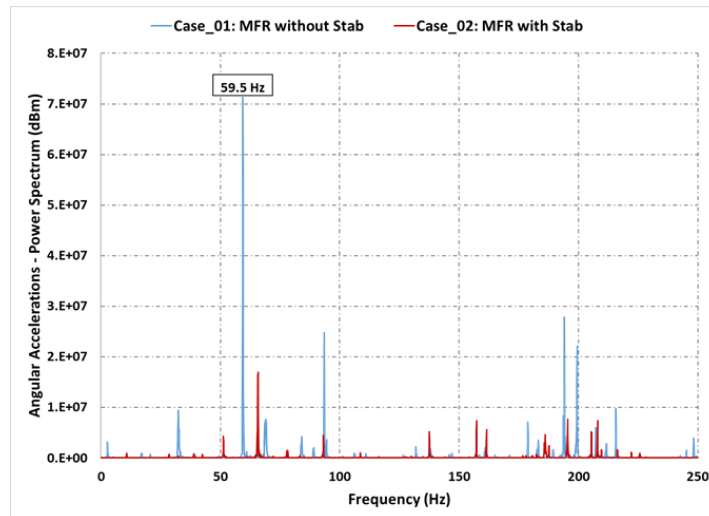
Figure 8. FFT of angular accelerations at center of RSS shaft.
