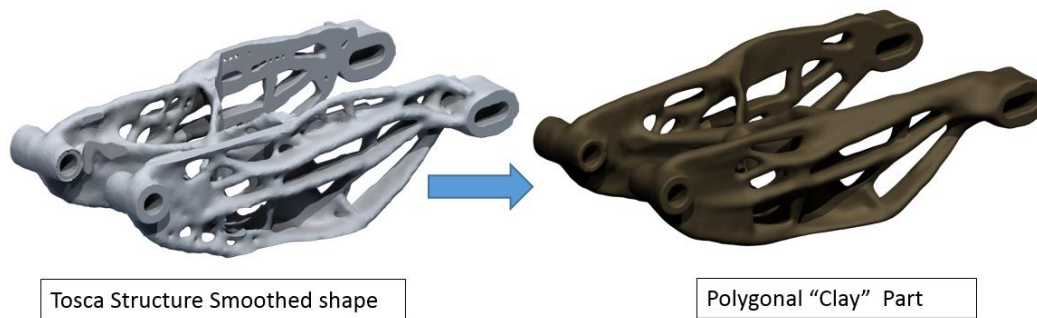
Figure 13. Polygonal clay part obtained from FEM
