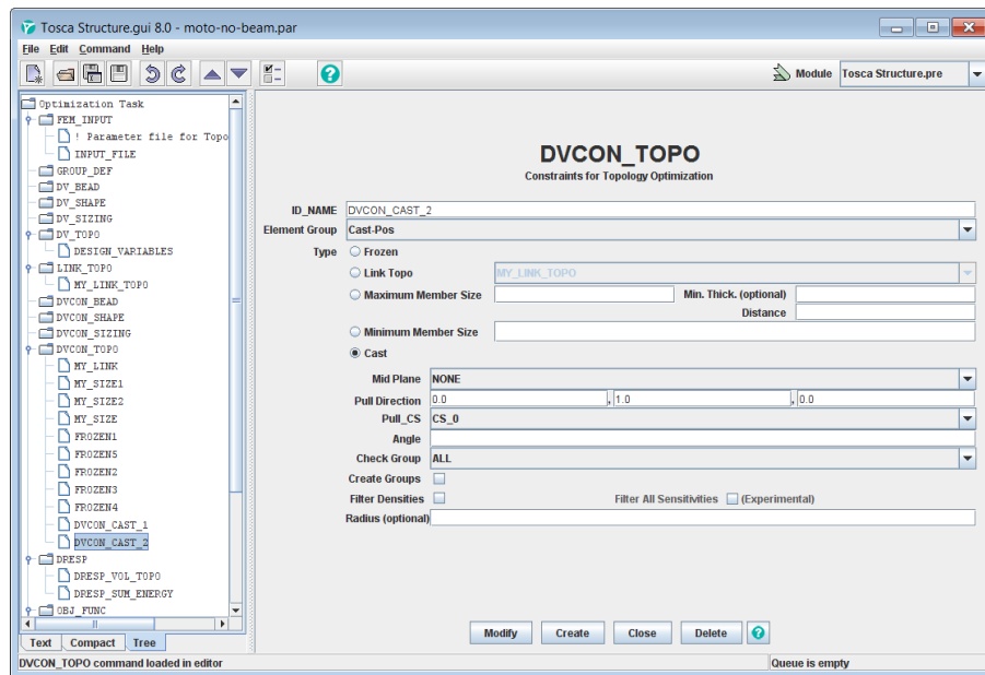
Figure 8. Casting Design Variable Constraint in Tosca Structure
