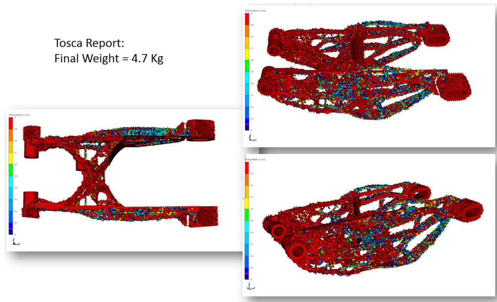
Figure 10. Swing arm optimized shape – Tosca Report View
