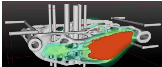
Figure 14. Casting virtual evaluation
