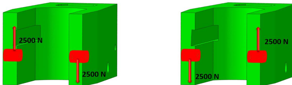
Figure 5. Load Case 1: Service loads acting on swing arm due to passenger load.
