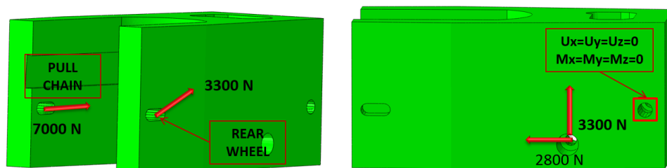
Figure 5. Load Case 1: Service loads acting on swing arm due to passenger load.
