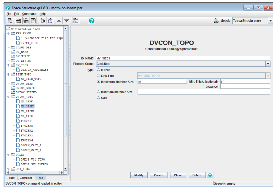
Figure 9. Maximum Member Size Constraint in Tosca Structure
