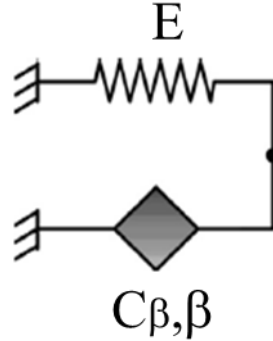
Figure 2. Fractional Kelvin-Voigt model
