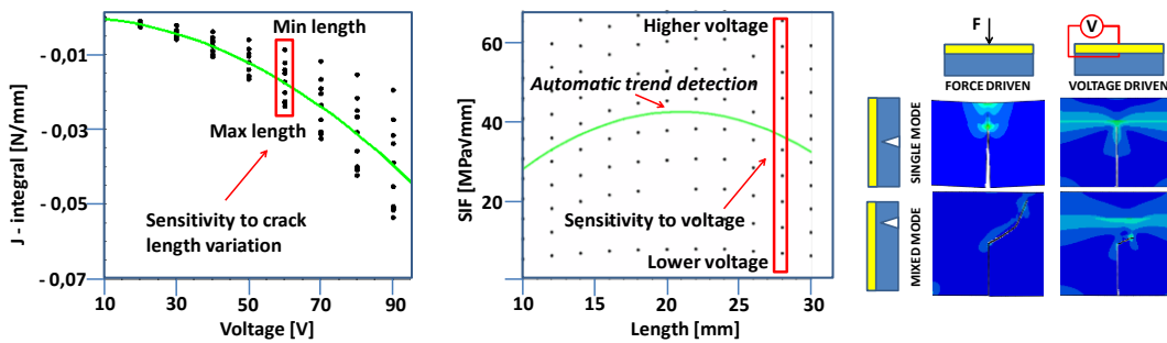
Figure 6. Relevant numerical results in voltage driven fracture of piezoelectric layer
