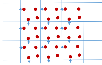
Figure 1. A 2-D periodic boundary condition cell.
