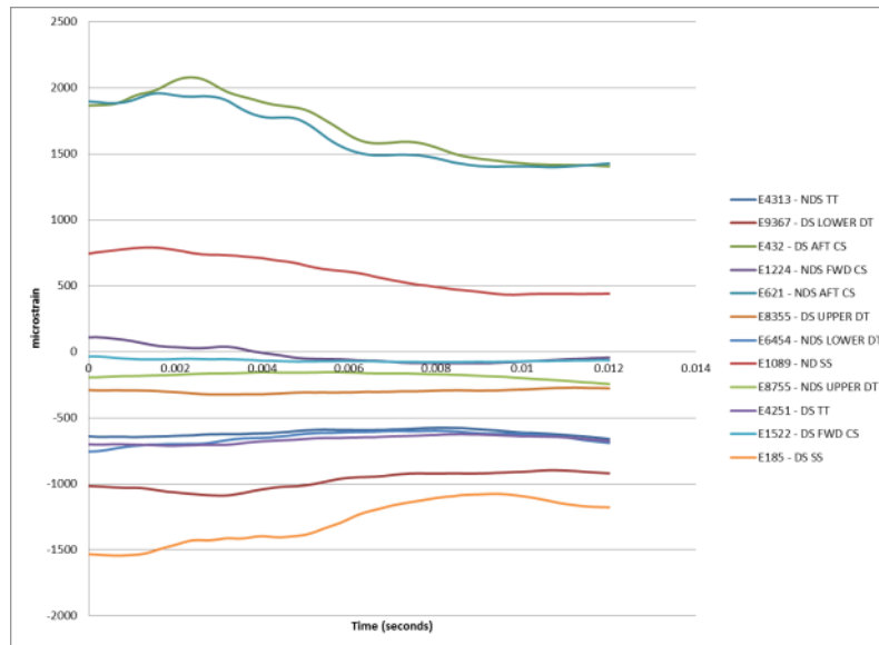
Figure 9. Strain gage data from Deer Hunter load case, 12 msec of data during impact where rear shock and front fork are in a near steady state configuration.
