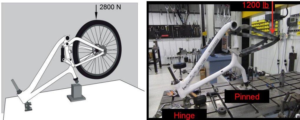
Figure 2. SS-EN ISO 4210-6 Tire clearance test and the Trek DOP test configurations.
