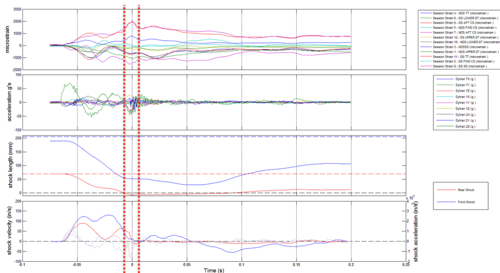
Figure 8. Sensor data from Deer Hunter landing case, data segment 23. Data starts with bicycle airborne. Note that shock velocity data are calculated data.
