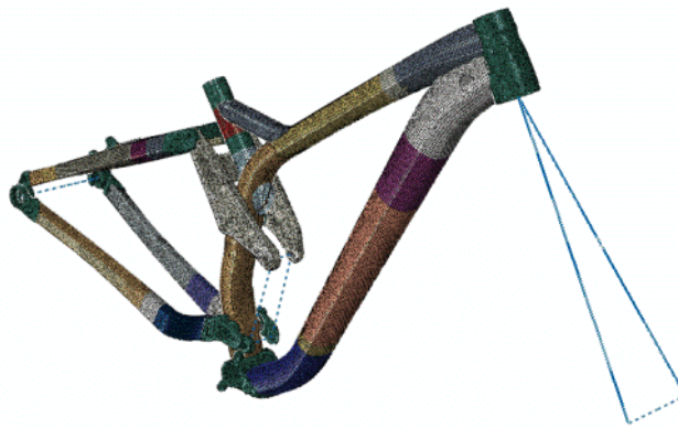
Figure 3. Aluminum Session 29er finite element model.
