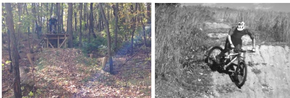
Figure 7. Deer Hunter straight drop landing load case (left) and Mojo “sideways” landing load case (right), Trek Trails.
