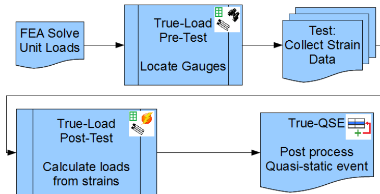
Figure 4. True-Load™ process flow.
