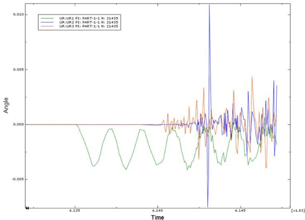
Figure 4-2. Rotational instability at a node in the inner pipeline as the loading exceeds F_c .
