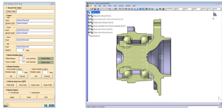
(a) CATIA template menu (b) Example of the analysis CAD model Figure 2. Example of CATIA template.
