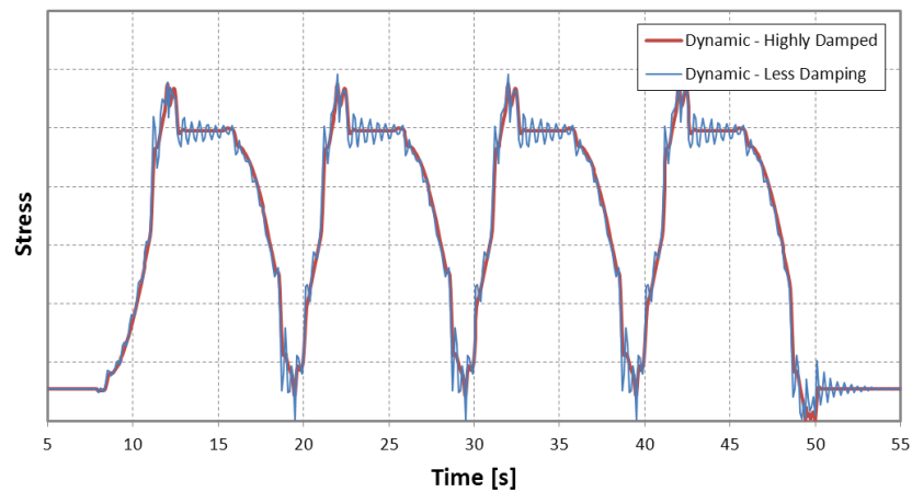
Figure 9. Stress History, Dynamic, High and Reduced Damping.
