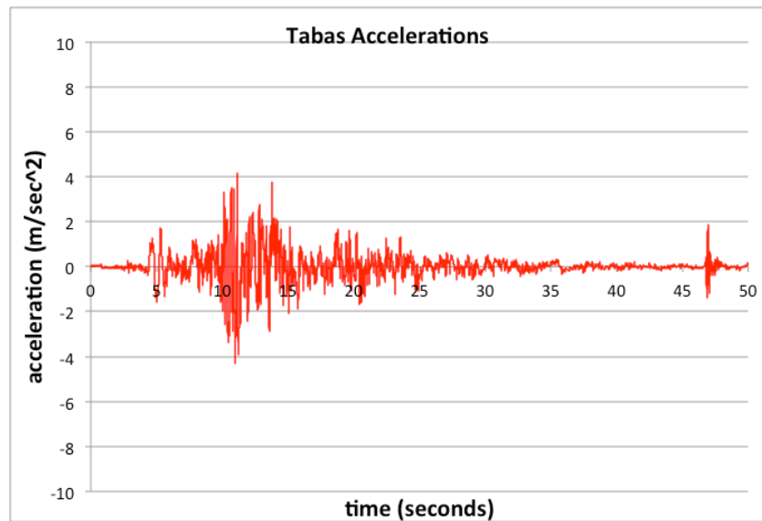
Figure 4 – Acceleration time histories for scaled TABAS earthquake.
