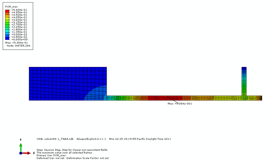
Figure 10 - Maximum hydrodynamic pressure distribution in case 4.
