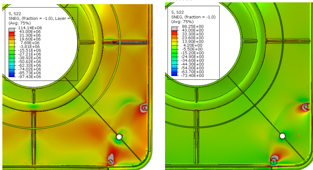
Fig 14. Diagram of principal Stress
