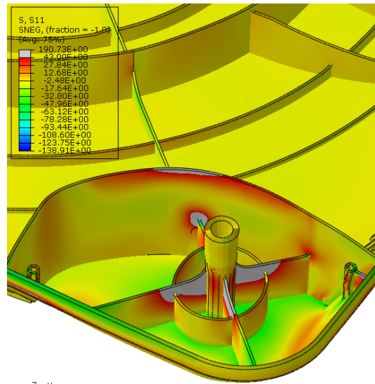
Fig 15. Diagram of principal Stress
