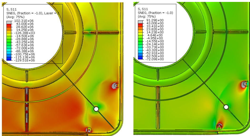
Fig 13. Diagram of principal Stress
