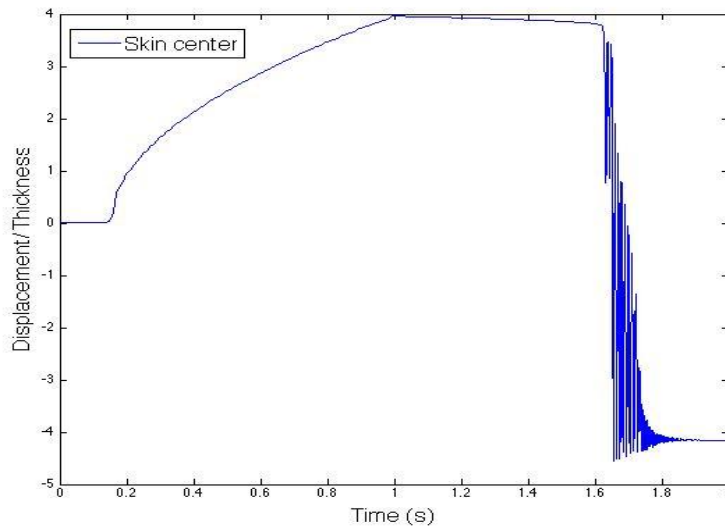
Figure 13. Reference points response when \Delta T = 200^\circ \text{F} , Pressure/ Time = 2
