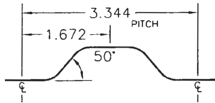
Figure 7. Profile of corrugated sheet door
