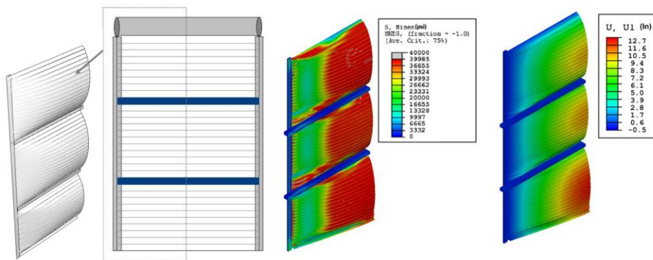
Figure 11. Door with two horizontal braces and von Mises stress and normal deflection fields for a 4" gap and 98 psf wind pressure
