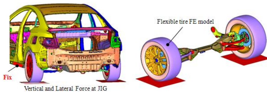
Figure 9. full FE model of the suspension system
