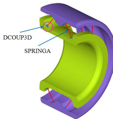
Figure 1. Bearing FE model
