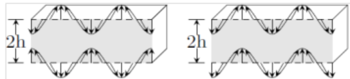
Figure 1. Lamb wave mode shapes; symmetric (left), anti-symmetric (right)
