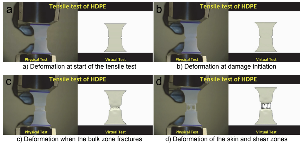
Figure 13. Experimental vs. Numerical results from tensile tests.
