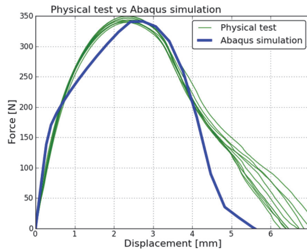
Figure 12. Tensile test results; experimental vs. numerical.
