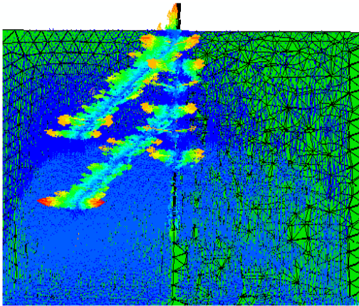
Stress distribution in root pattern A
