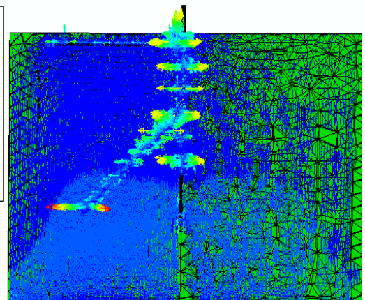
Stress distribution in root pattern M
