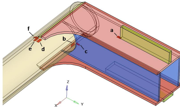
Figure 15. Selected sensor elements
