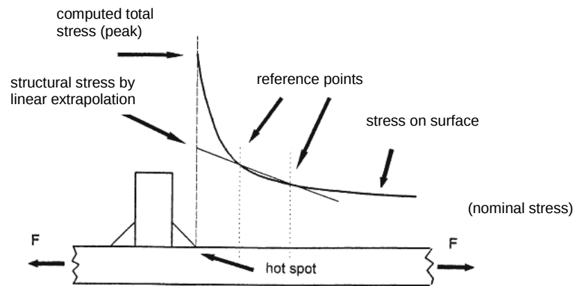
Figure 2. Stresses at welded joint (Hobbacher, 2007)
