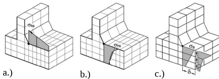
Figure 5. Different approaches for structural hot spot stresses (Fricke, 2005)
