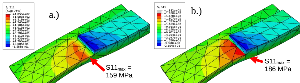
Figure 6. a) Averaged and b) non averaged results, doubling plate, coarse mesh
