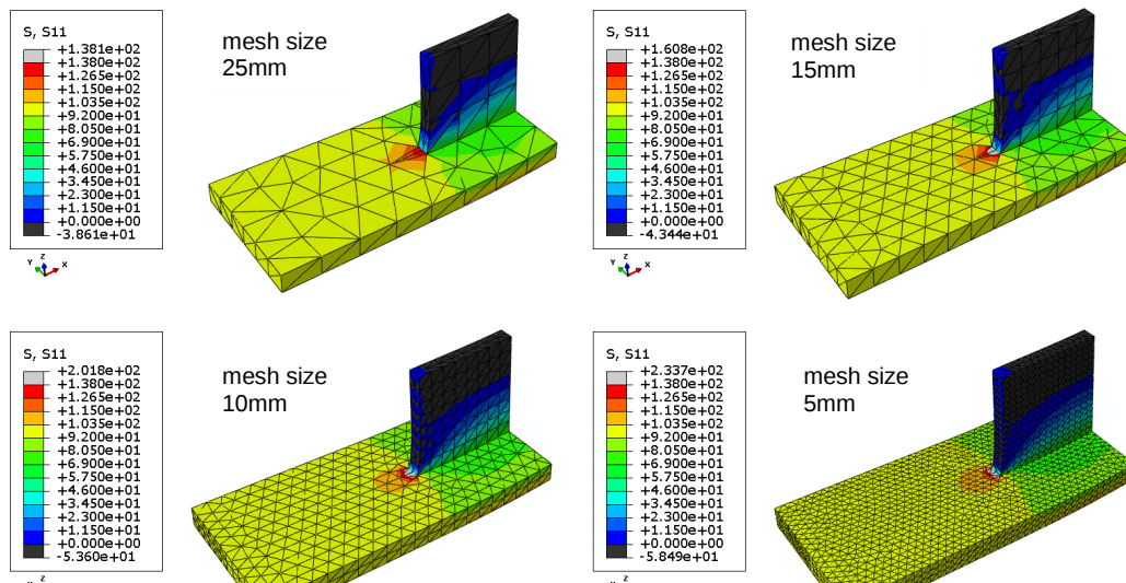
Figure 9. Flange with gusset, results for different mesh sizes
