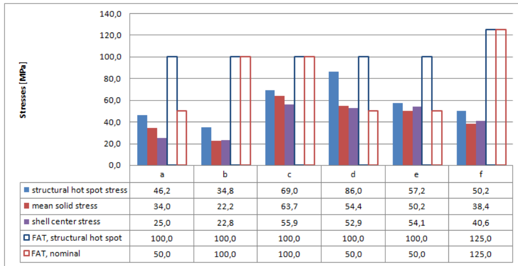
Figure 16. Stresses at different positions of welded assembly
