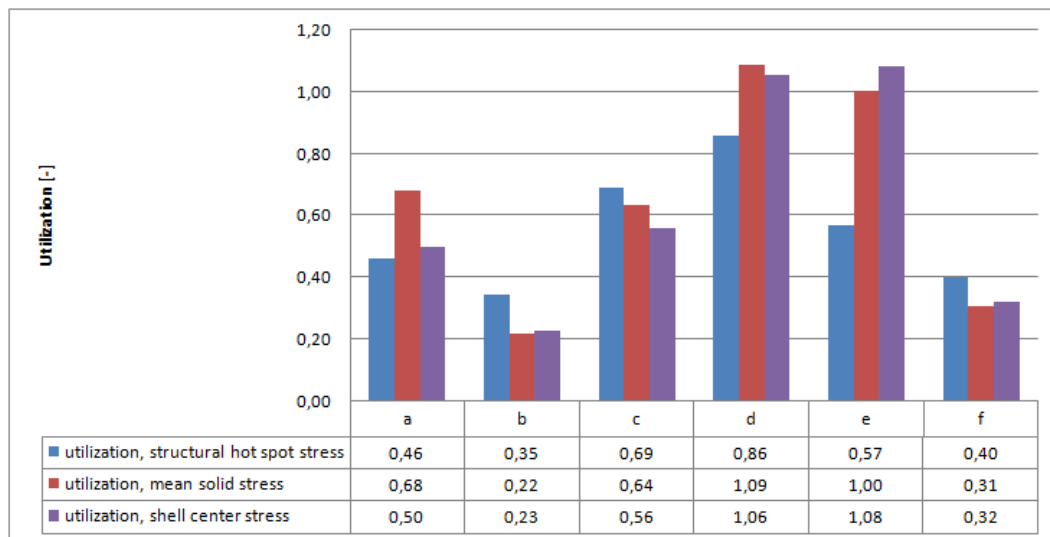
Figure 17. Utilization factors at different positions of welded assembly
