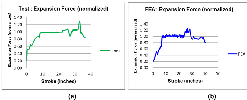
Figure 14. Lab Test vs FEA correlation
