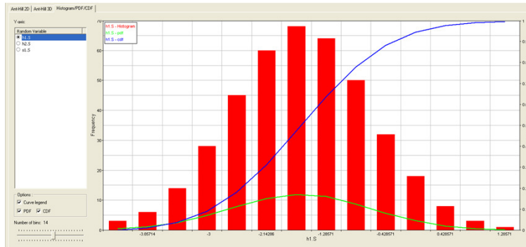
Random Variable Histogram/PDF/CDF
