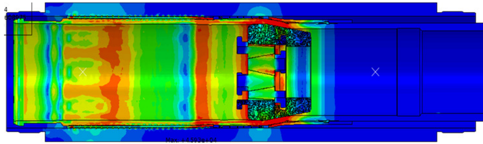
Figure 8. Stress plot
