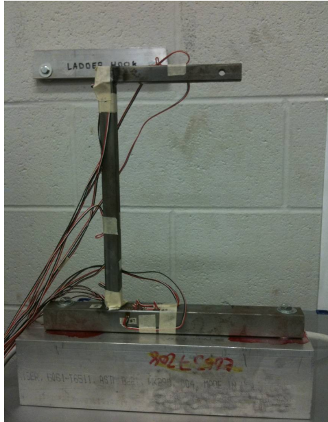
Figure 1: Hangman Fixture
