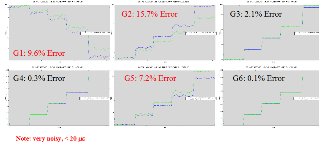
Figure 6: Experimental & Analytical Strain Signals
