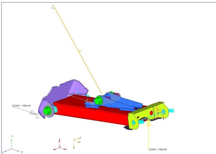
Figure9: FE modeling of the Simplified suspension assembly
