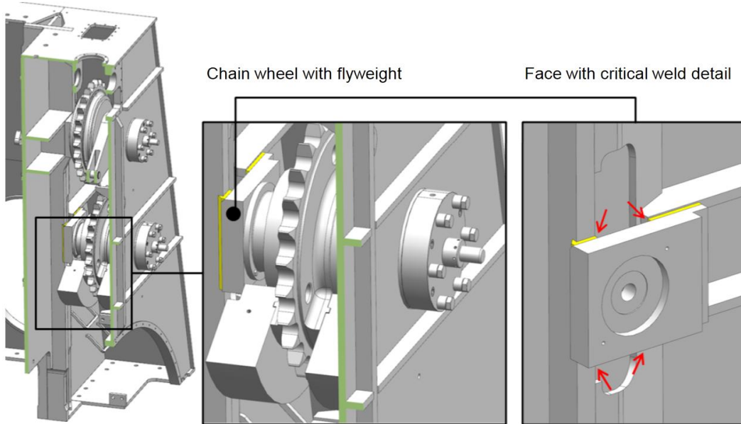
Figure 5: Critical weld detail illustrated on chain wheel with flyweight for the second order moment compensator.
