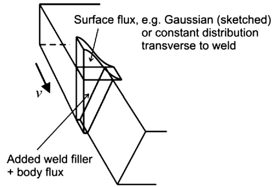
Figure 3. Principle of moving heat source for welding, modelled with addition of weld filler, a body flux and a surface flux shown on symmetric half of a butt weld.
