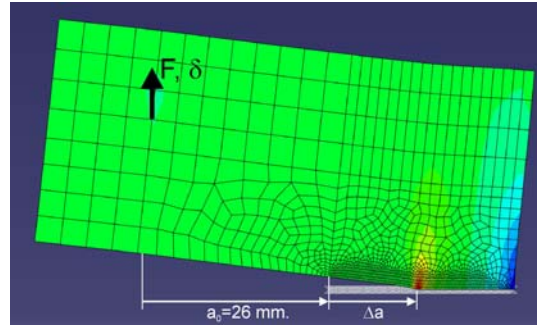
Figure 5. Shell model of Compact Tension Specimen with cohesive elements for fracture.
