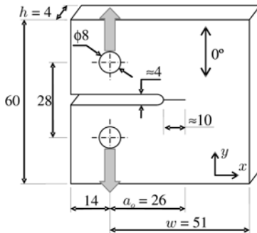
Figure 4. Compact Tension Specimen (after Pinho, et al., 2006).
