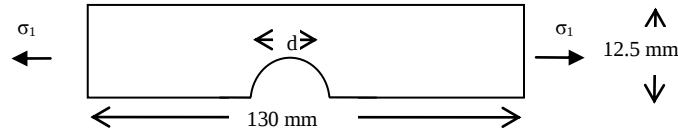
Figure 1. Geometry dimensions of notched composite plate (after Belmonte et. al, 2001, 2004).
