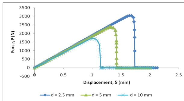
Figure 4: Typical load-displacement plot implementing CZM approach of (0/90/\pm 45)_s lay-up
