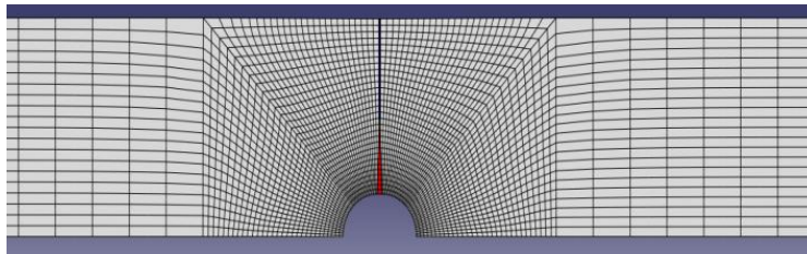
Figure 3. Crack propagation from notch edge using CZM
