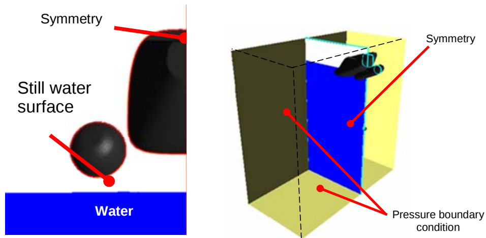
Figure 7 CFD model of helicopter splashdown.
