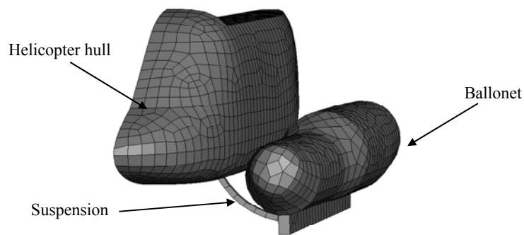
Figure 6 Helicopter finite-element model (one-half)
