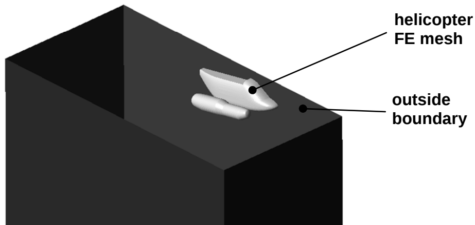
Figure 2 Boundaries of fluid computational domain.
