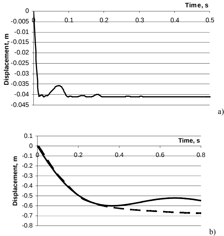
Figure 9 Vertical displacement of helicopter center mass. a) Landing. b) Splashdown; solid line – rigid ballonets; dashed line – deformed ballonets
