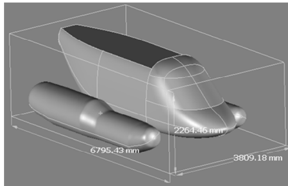
Figure 5 Helicopter model
