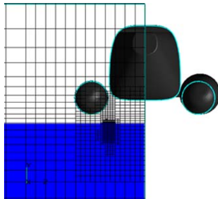
Figure 8 Finite-volume mesh with local adaptation near hull and ballonets.
