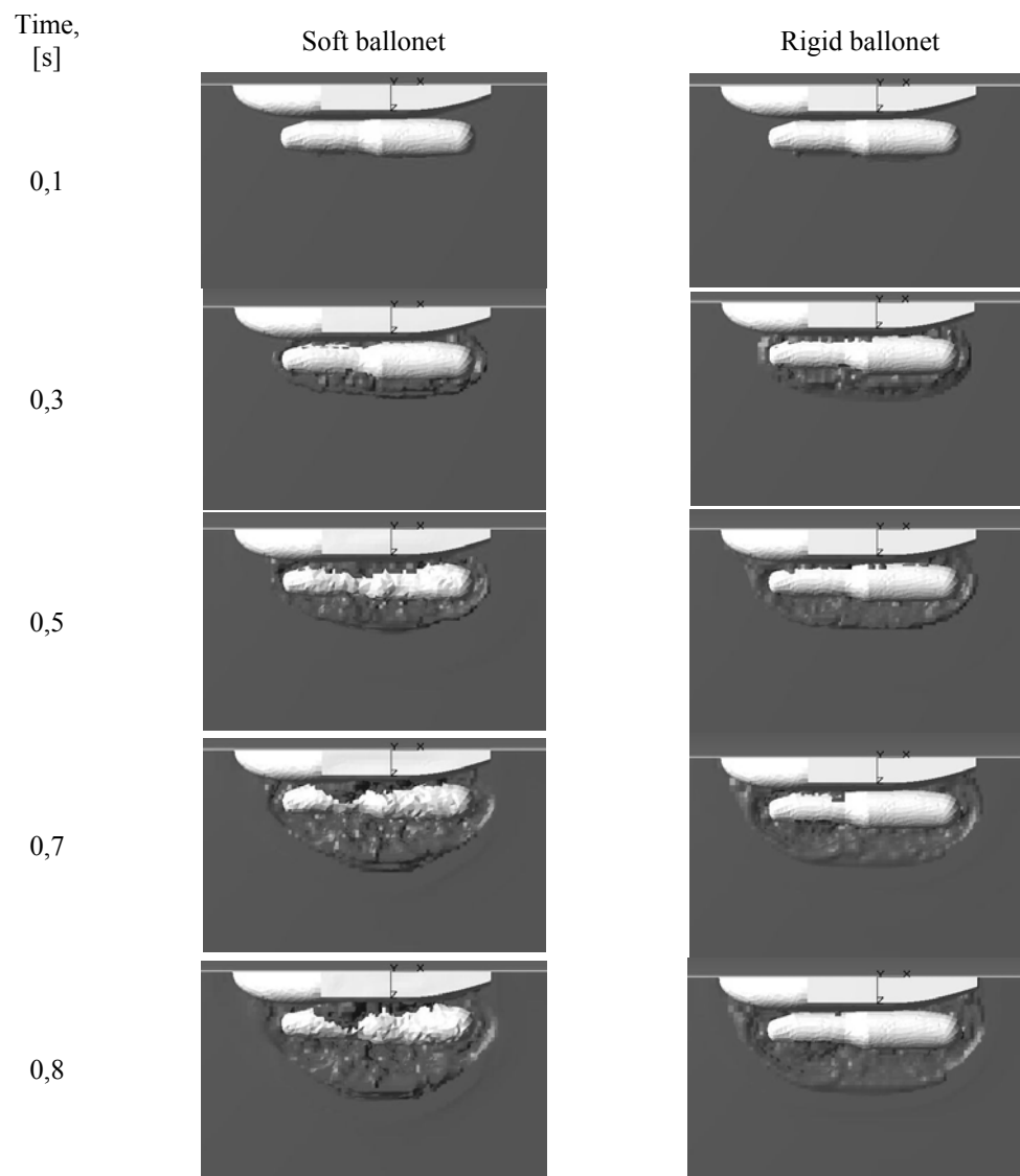
Figure 12 Comparison of water distribution over the helicopter for rigid and soft ballonets.
