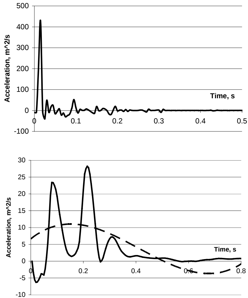
Figure 10 Vertical acceleration of helicopter center mass. a) Landing. b) Splashdown; solid line – rigid ballonets; dashed line – deformed ballonets
