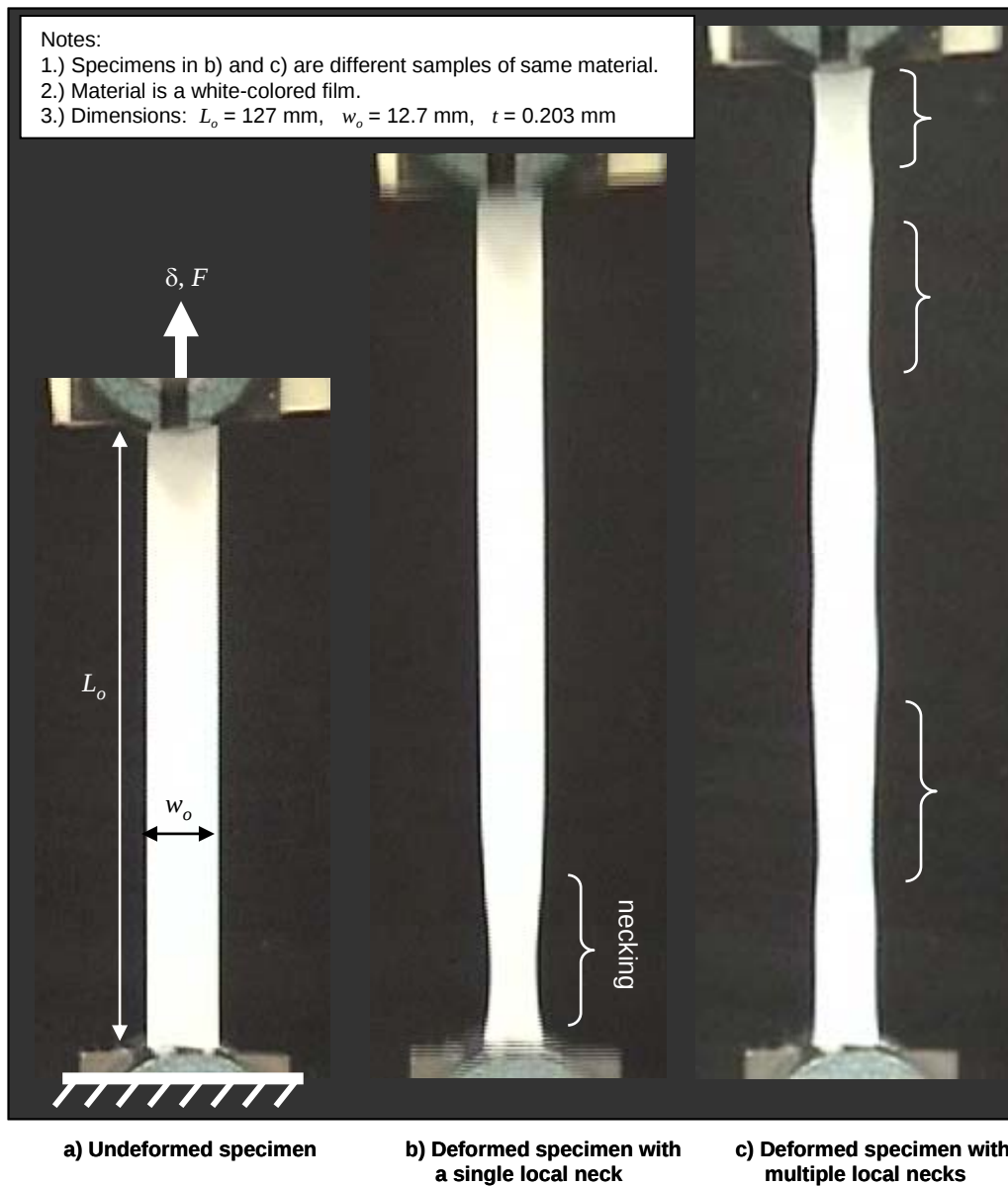
Figure 1: Examples of localized necking in uniaxial tensile tests of Obermühle Ö-Colamin “MP” Flachfiol Film.
