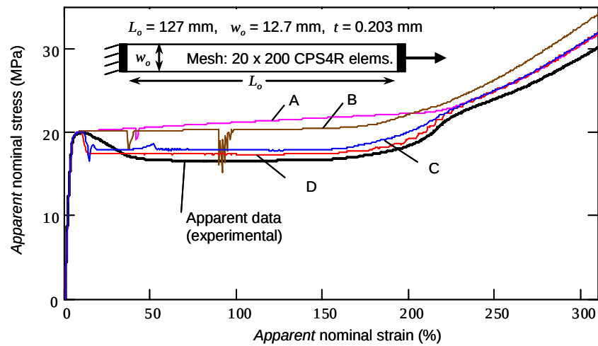
b) Apparent nominal stress/strain curves derived from ABAQUS/Explicit simulation data
