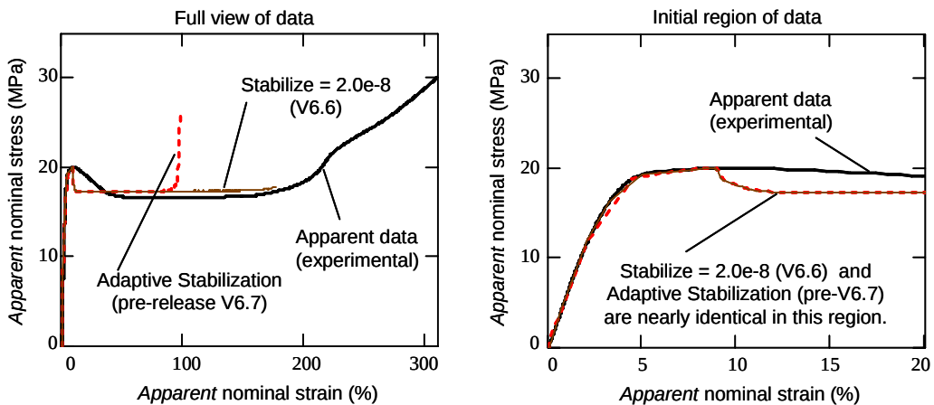
b) Results derived from ABAQUS/Standard V6.6 simulation data using non-default stabilization parameter value and from ABAQUS/Standard V6.7 pre-release using new adaptive stabilization algorithm.
