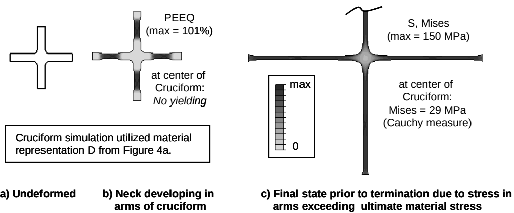
Figure 6: ABAQUS/explicit predictions of biaxial response for cruciform loading.
