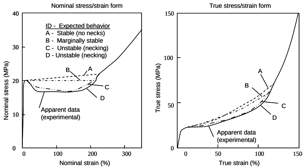
a) Stress/Strain curves used to generate *Elastic and *Plastic data for ABAQUS simulations
