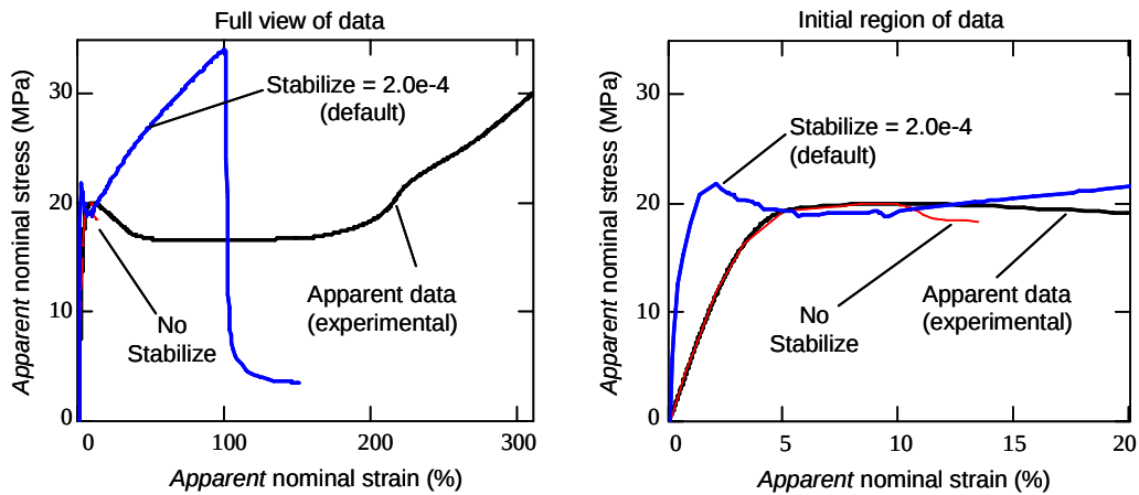
a) Results derived from ABAQUS/Standard V6.6 simulation data without stabilization and with stabilization (using default parameter value).
