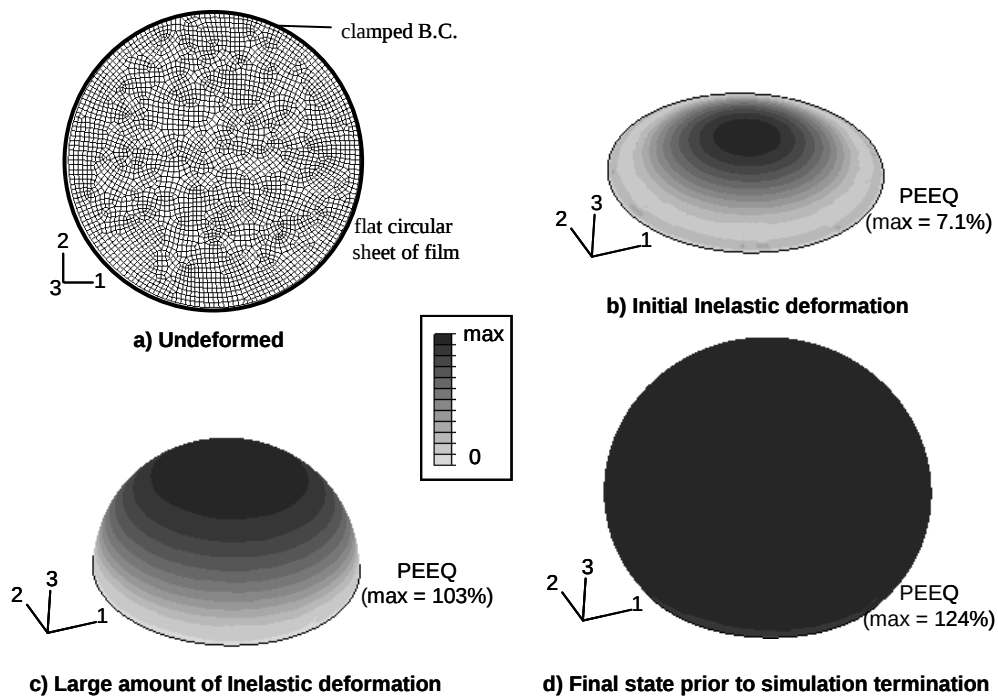
Figure 7: ABAQUS/explicit predictions of inflation of a flat circular sheet utilized material representation D from Figure 4a.
