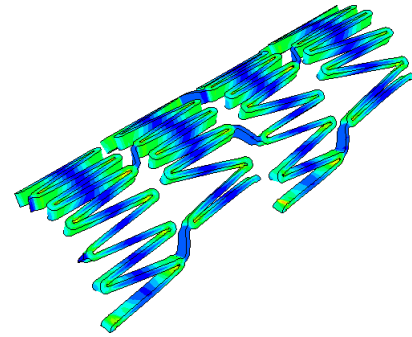
Figure 6: Crimped stent.
