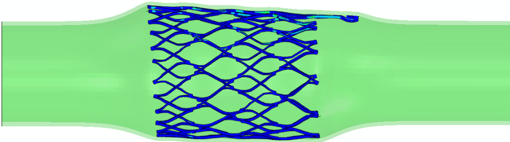
Figure A-2. Deformed configuration of a proximal anchor embedded in a hyperelastic tube with Krams material parameters at 10mm Hg internal pressure.
