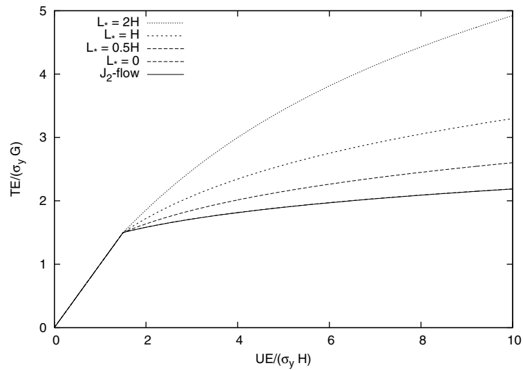
Figure 2. The shear response found for an infinite wide slab with full constrain of the plastic strain along the horizontal boundaries.
