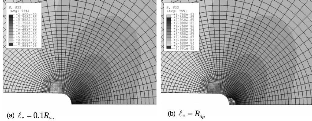
Figure 7. The contours of the horizontal stress components \sigma_{22}
