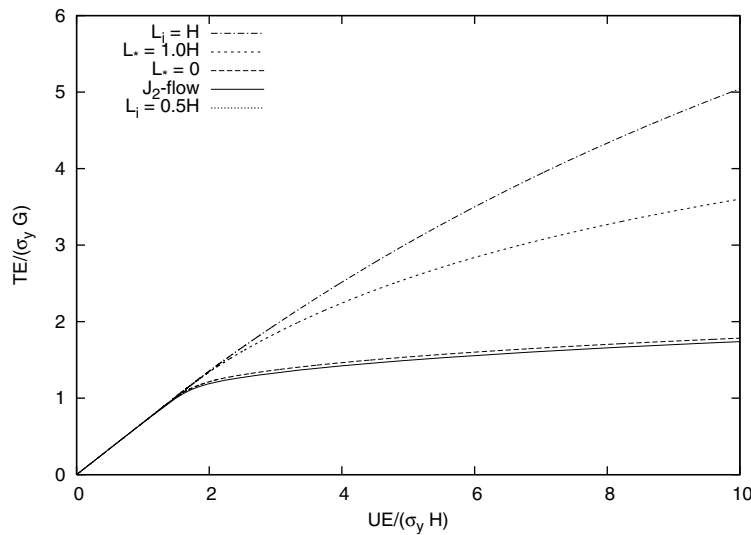
Figure 5. The shear response found for a finite wide slab W / H = 1 with full constrain of the plastic strain along the horizontal boundaries.
