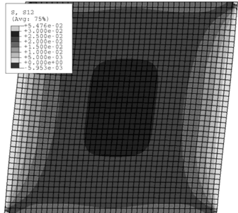
(b) Enhanced plasticity model \ell_* = 0
