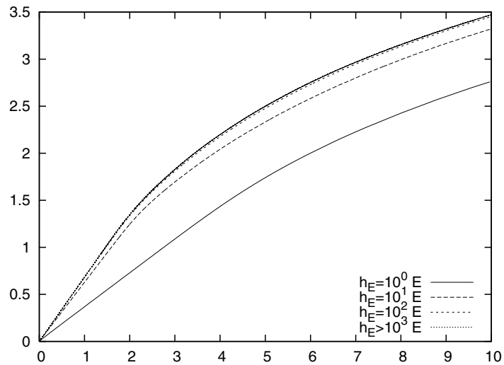
Figure 6. The shear response found for a finite wide slab W / H = 1 with full constrain of the plastic strain along the horizontal boundaries.
