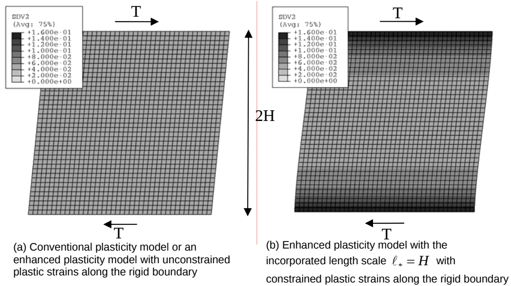
Figure 1. Infinite wide slab sheared between two horizontal rigid boundaries.
