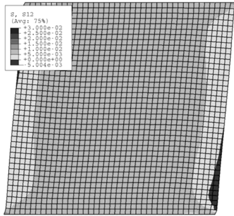
(a) Conventional plasticity model
