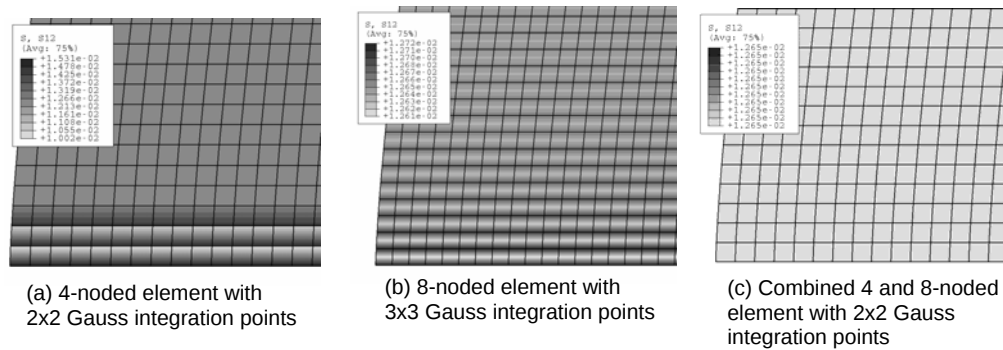
Figure 3. Zoom in on the bottom left corner of the contour plots of the shear stresses as a function of the chosen element type.
