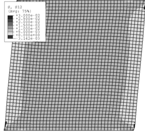
(b) Enhanced plasticity model \ell_* = 0
