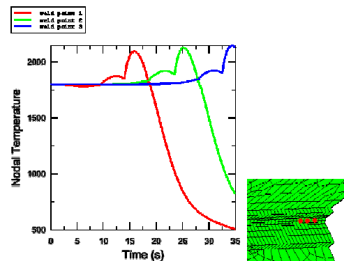
Figure 3: Transient temperature profile at three points in the torch path
